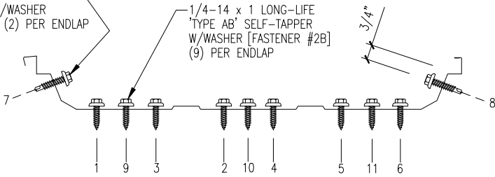
FASTENER SEQUENCE @ ENDLAP
