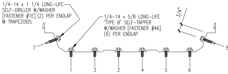
FASTENER SEQUENCE @ ENDLAP
