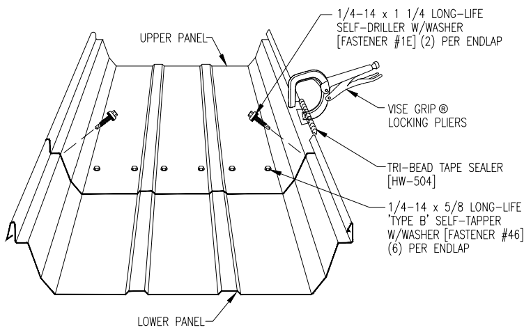
PANEL INSTALLATION SEQUENCE
