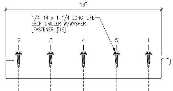
FASTENER INSTALLATION SEQUENCE
