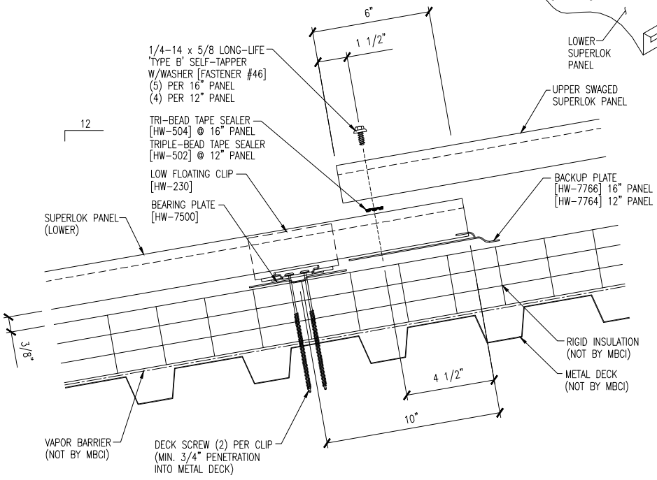
FASTENER INSTALLATION SEQUENCE
