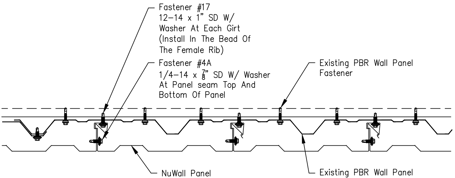
Retrofit NuWall Panel Attachment
