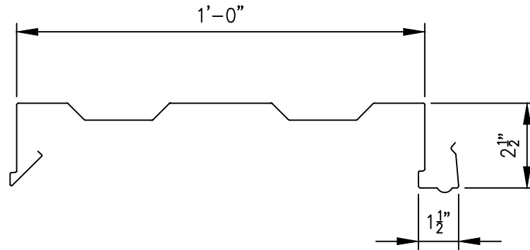
NuWall Panel Profile
