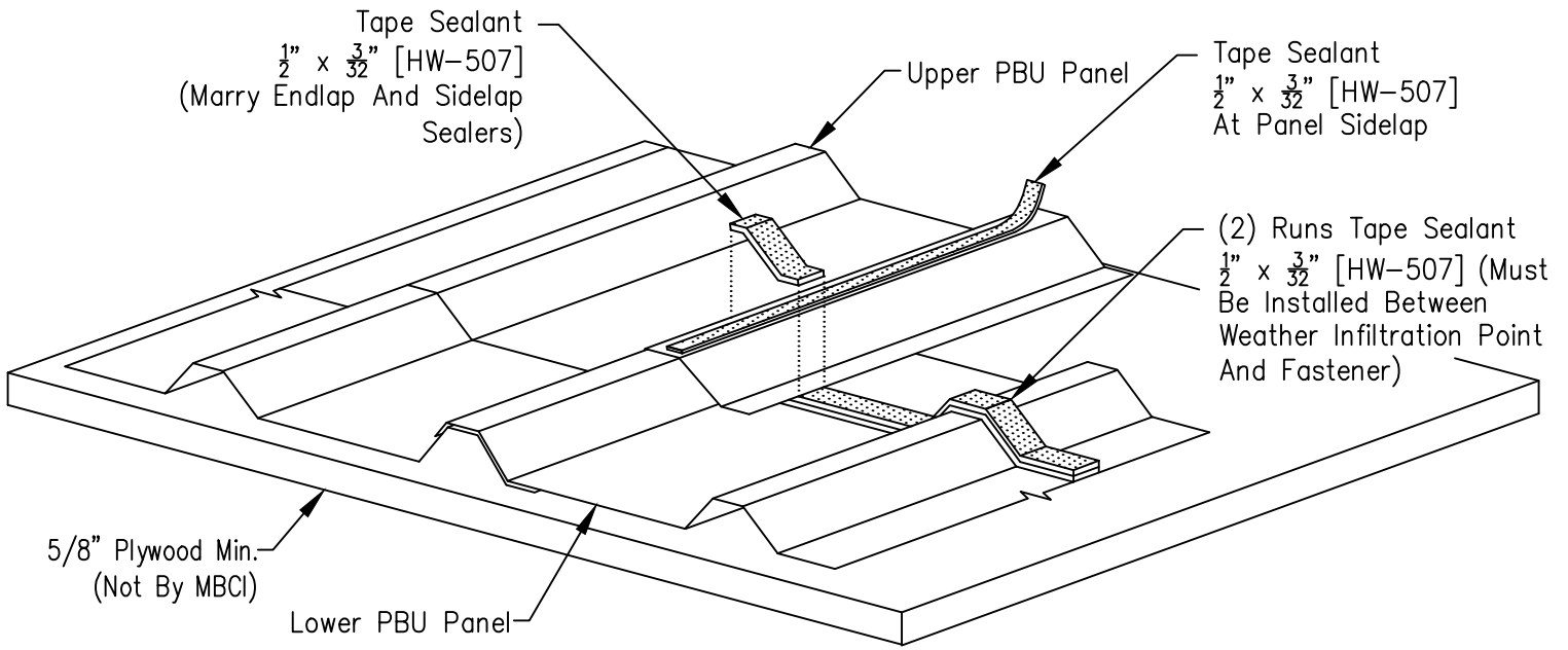
Endlap Sealant Detail
