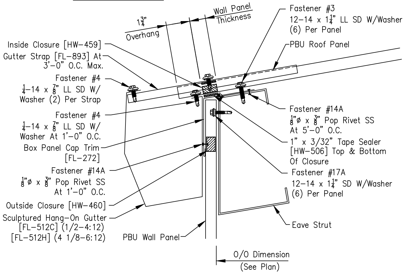
Eave Sealant Detail
