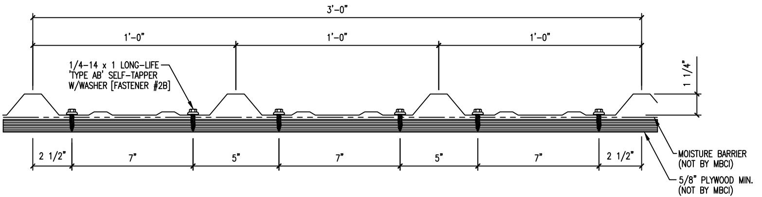
PBR FASTENER SPACING @ PANEL ENDS
