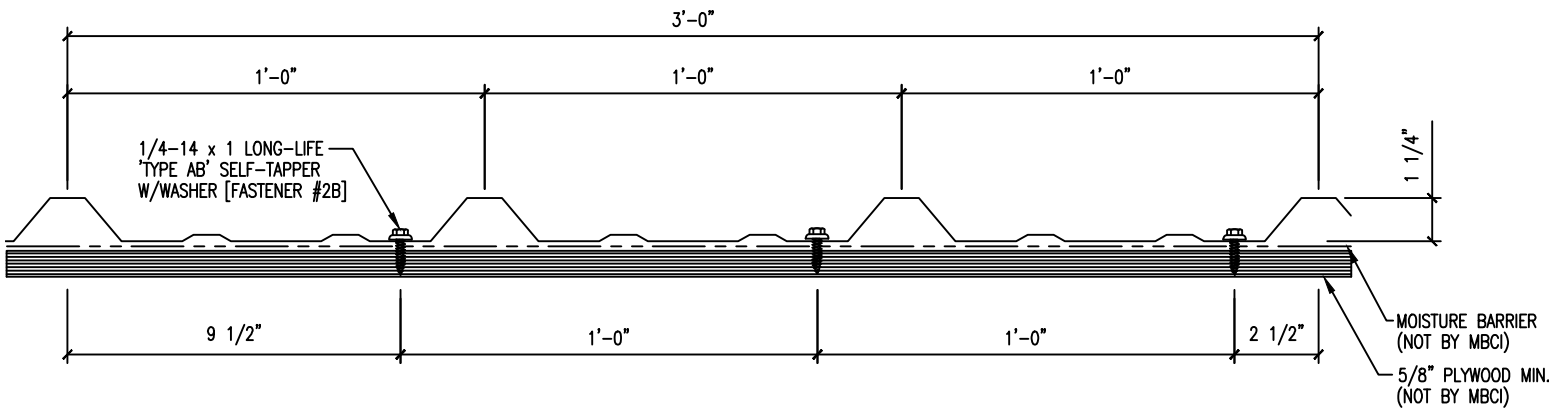
PBR FASTENER SPACING @ INTERMEDIATE SUPPORTS
