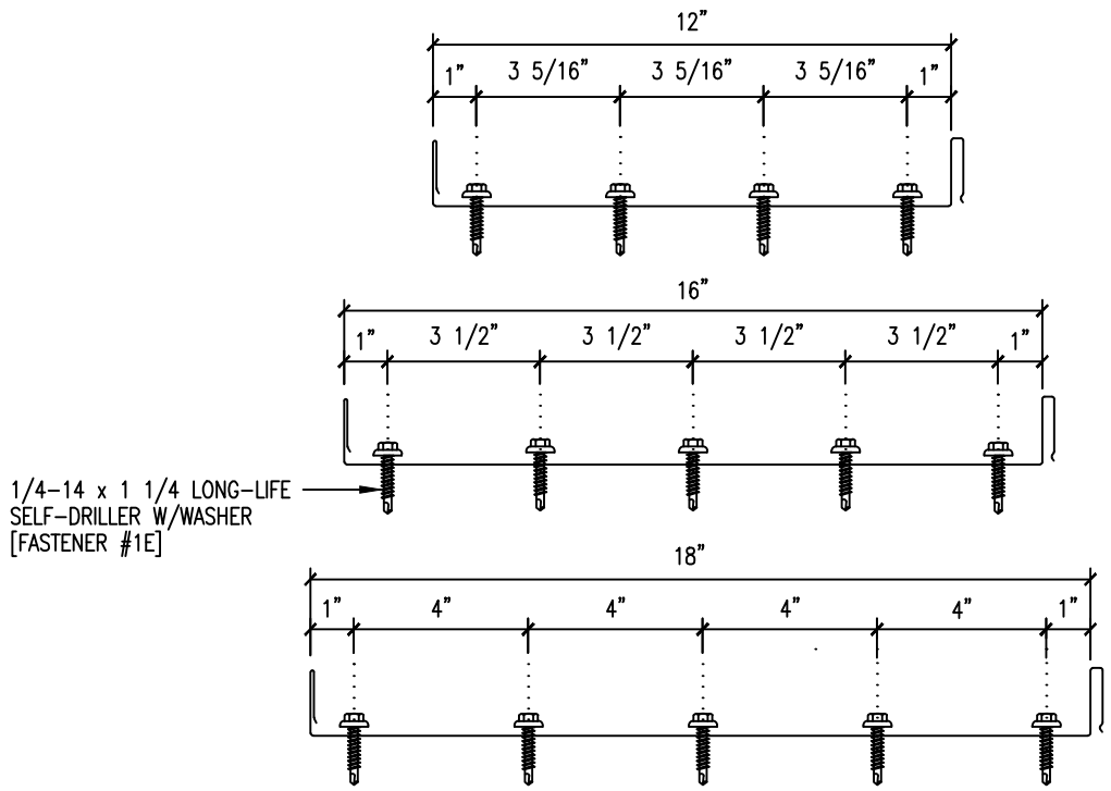
FASTENER SPACING @ EAVE
