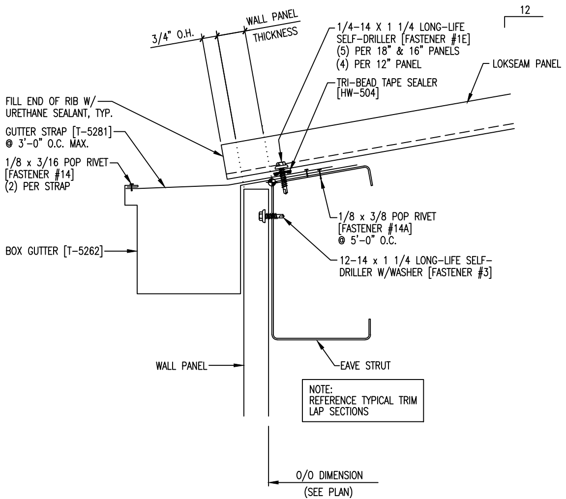
FASTENER SPACING @ EAVE
