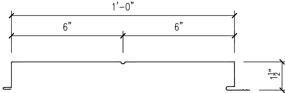
FW-120-1 PANEL PROFILE W/ BEAD
