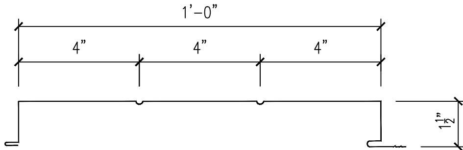
FW-120-2 PANEL PROFILE W/ BEADS
