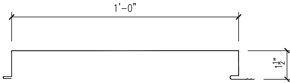
FW-120-0 PANEL PROFILE
