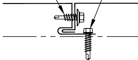
PANEL SIDELAP
