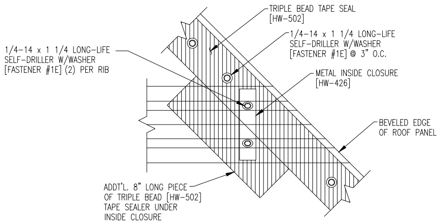
DETAIL "A"
