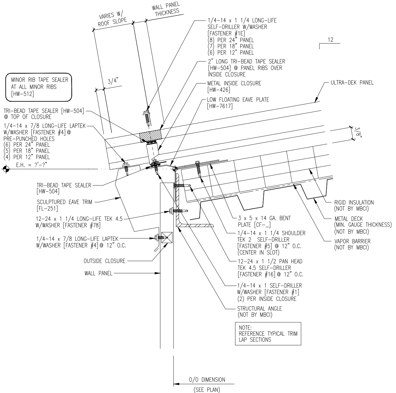
FASTENER SEQUENCE @ EAVE
