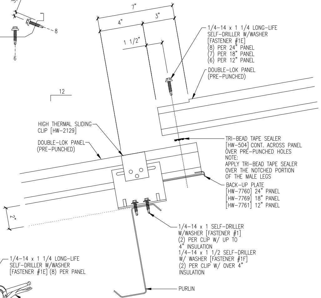
FASTENER SEQUENCE @ ENDLAP
