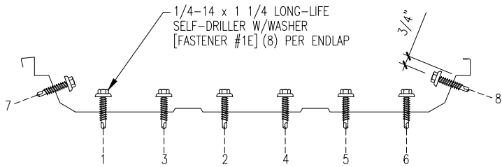
FASTENER SEQUENCE @ ENDLAP
