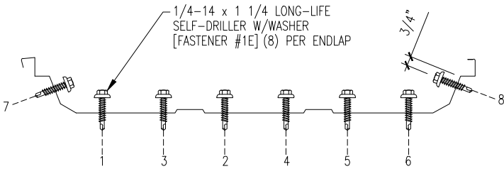
FASTENER SEQUENCE @ ENDLAP
