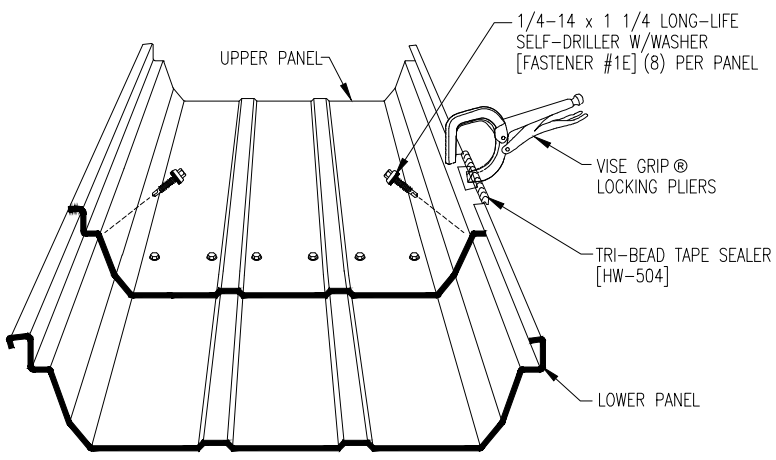
PANEL INSTALLATION SEQUENCE
