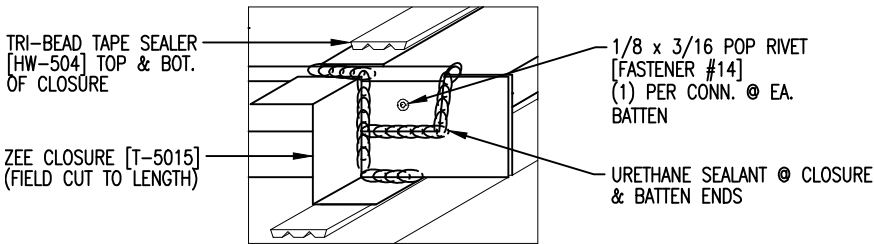
HIGH EAVE SEALANT DETAIL
