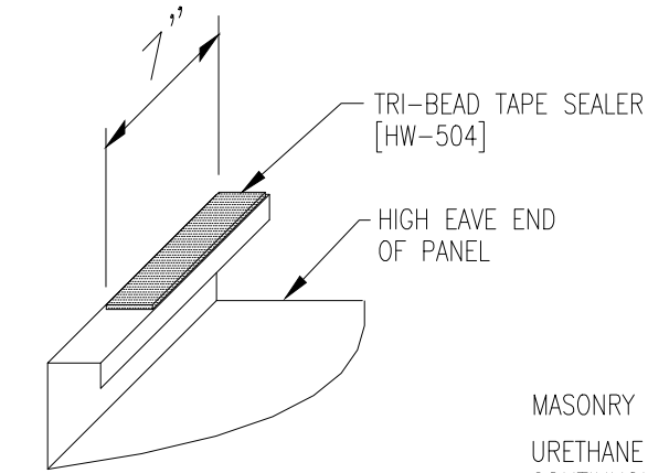
HIGH EAVE SEALANT DETAIL
