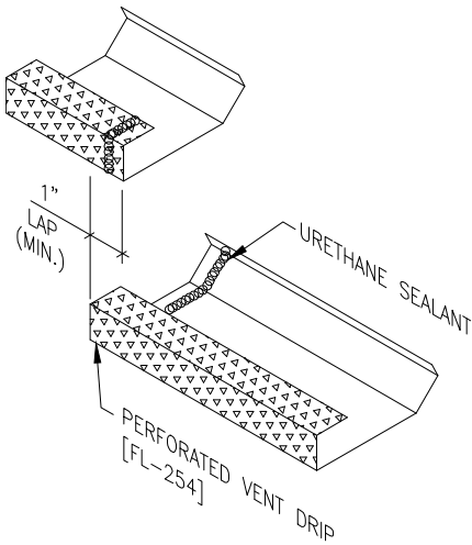
HIGH EAVE SEALANT DETAIL
