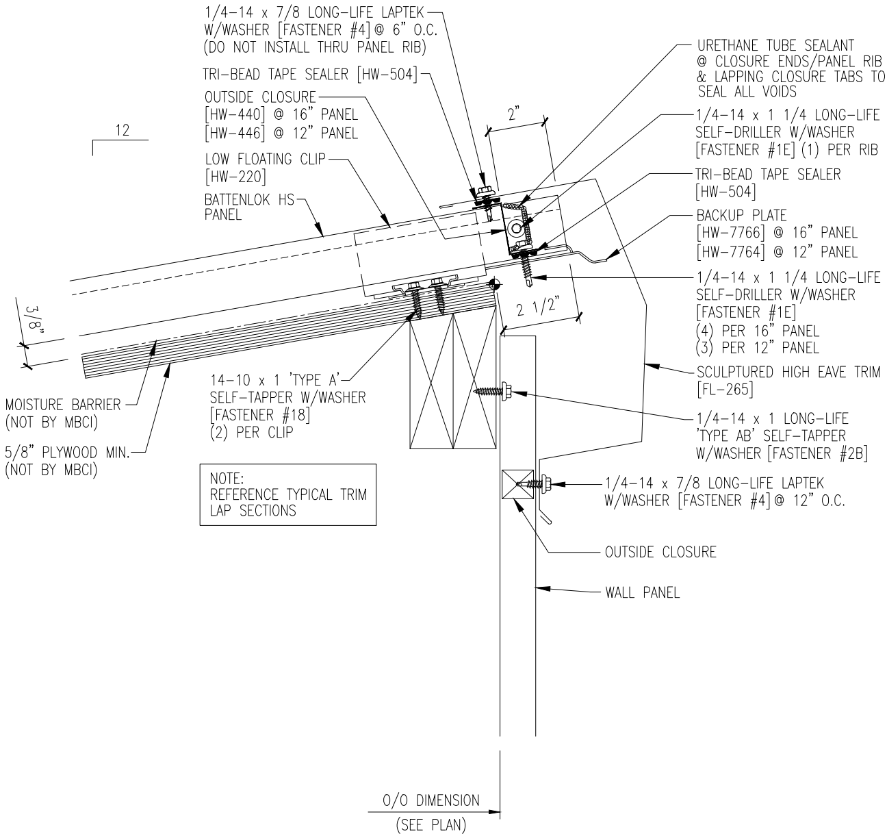
HIGH EAVE SEALANT DETAIL
