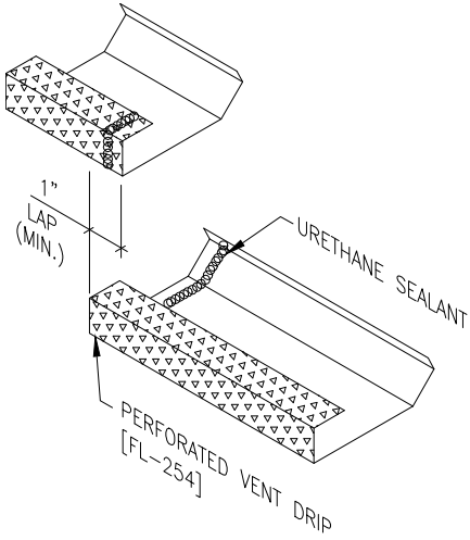
HIGH EAVE SEALANT DETAIL
