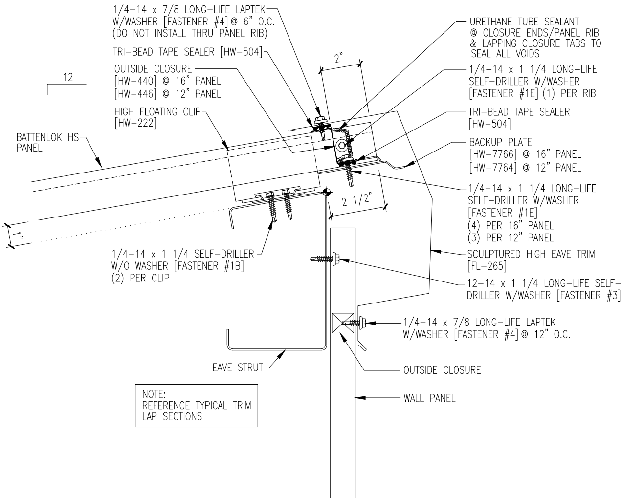
HIGH EAVE SEALANT DETAIL
