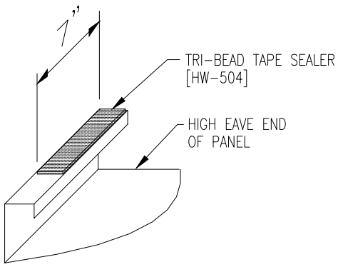
HIGH EAVE SEALANT DETAIL
