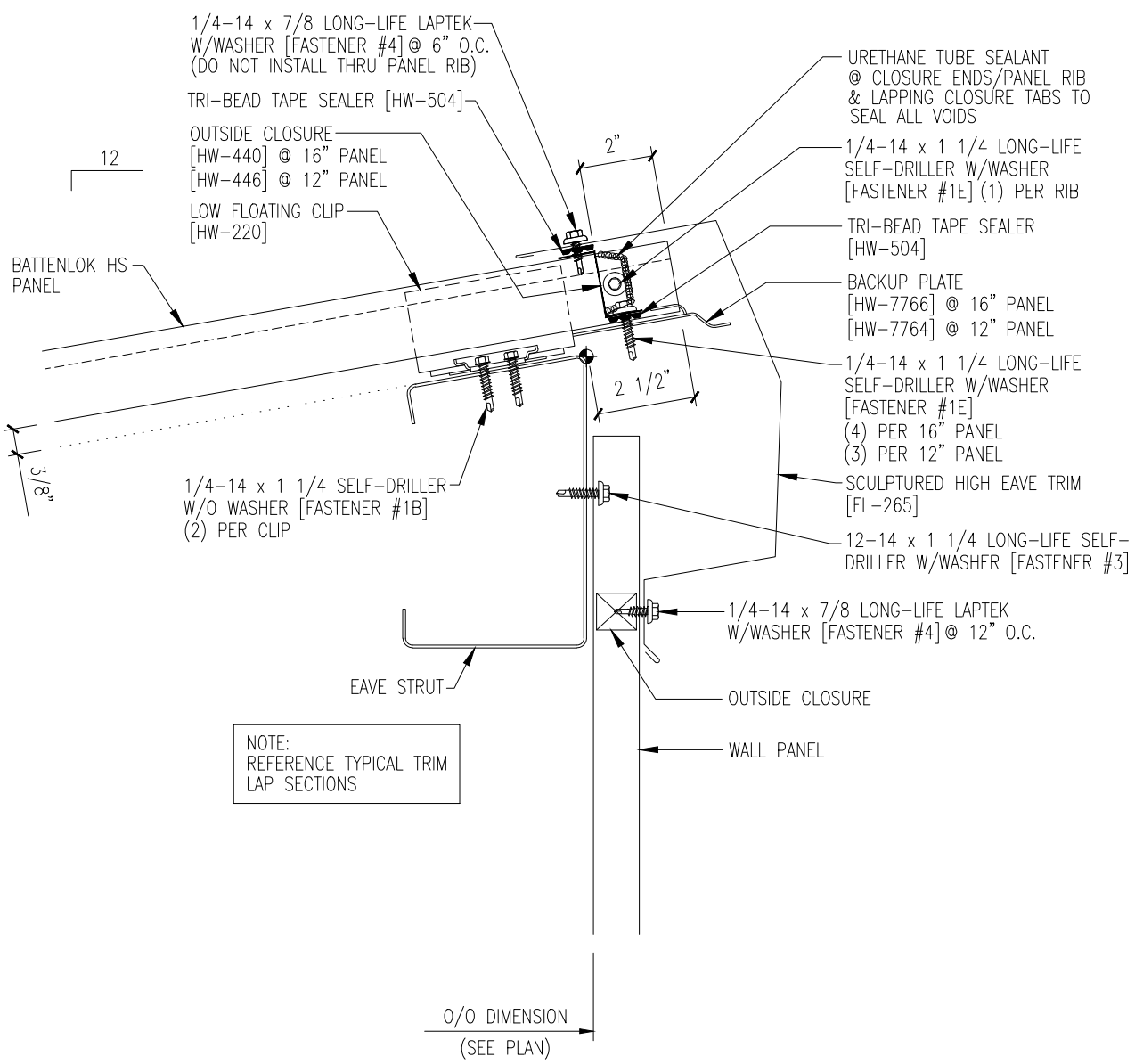
HIGH EAVE SEALANT DETAIL
