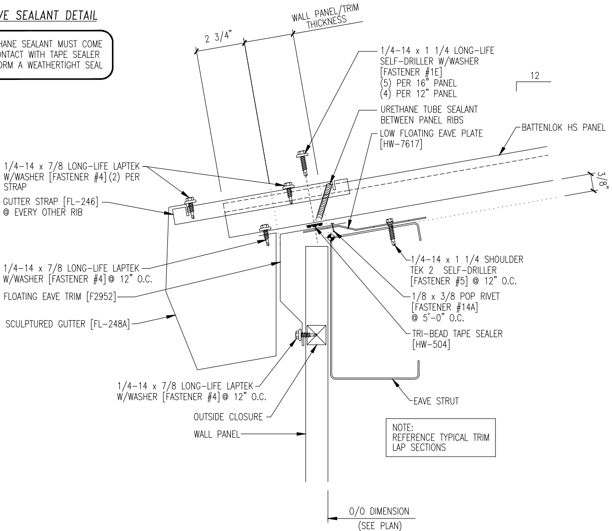
FASTENER SPACING @ EAVE
