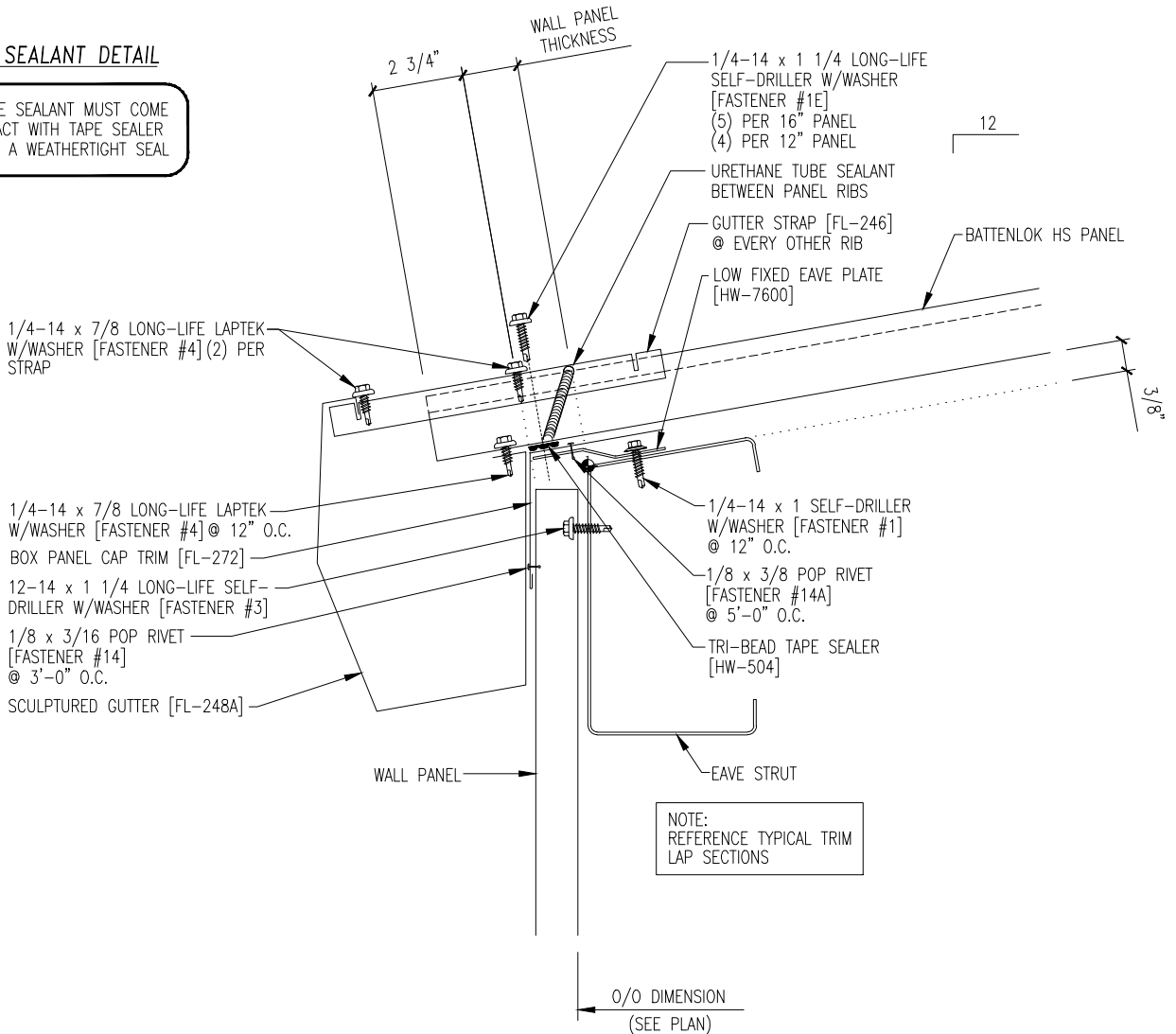
FASTENER SPACING @ EAVE
