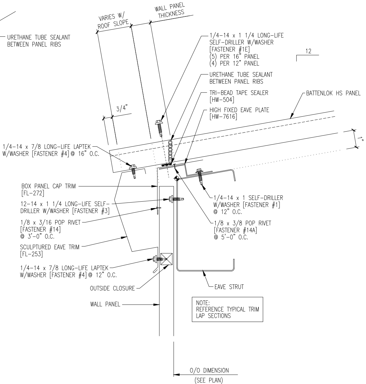
EAVE SEALANT DETAIL
