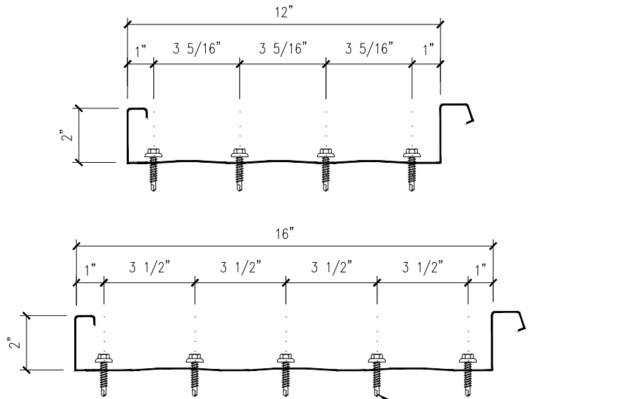
FASTENER SPACING @ EAVE
