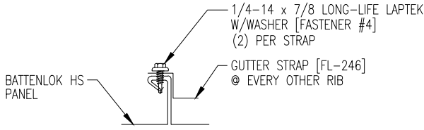
GUTTER STRAP ATTACHMENT
