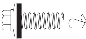
12-14 x 1" Driller \frac{5}{16} " Hex Washer Head w/ \frac{5}{8} " O.D. Washer
