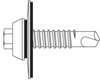
1/4"-14 x 1 1/4" Long Life Driller 5/16" Hex Washer Head w/ 1 1/8" O.D. Washer
