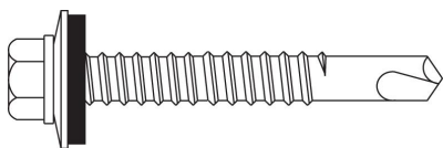
12-14 x 1\frac{1}{2} " Driller \frac{5}{16} " Hex Washer Head w/ \frac{5}{8} " O.D. Washer
