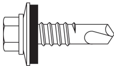
12-14 x \frac{3}{4} " Driller \frac{5}{16} " Hex Washer Head w/ \frac{5}{8} " O.D. Washer
