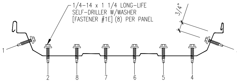
FASTENER SEQUENCE @ EAVE
