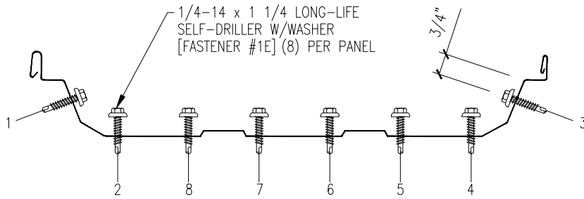
FASTENER SEQUENCE @ EAVE
