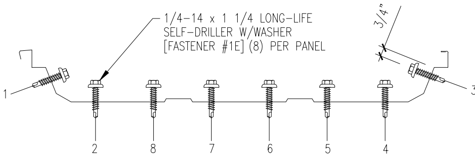
FASTENER SEQUENCE @ EAVE
