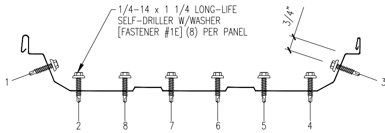
FASTENER SEQUENCE @ EAVE
