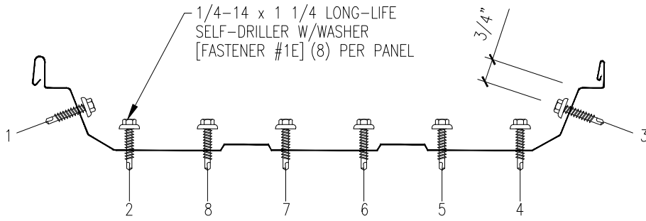
FASTENER SEQUENCE @ EAVE
