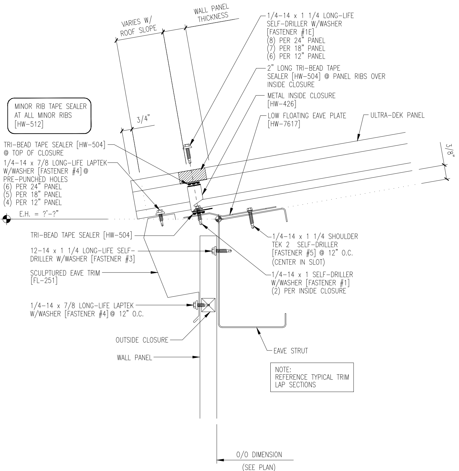
FASTENER SEQUENCE @ EAVE
