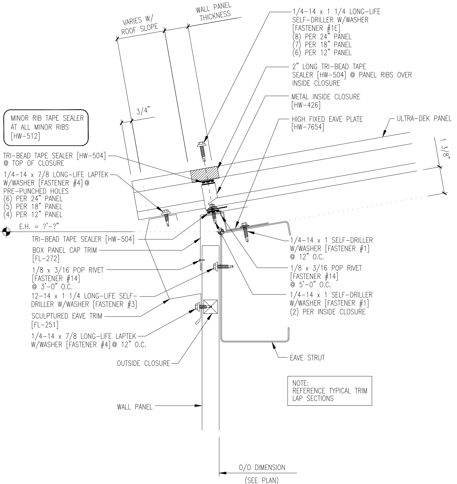
FASTENER SEQUENCE @ EAVE
