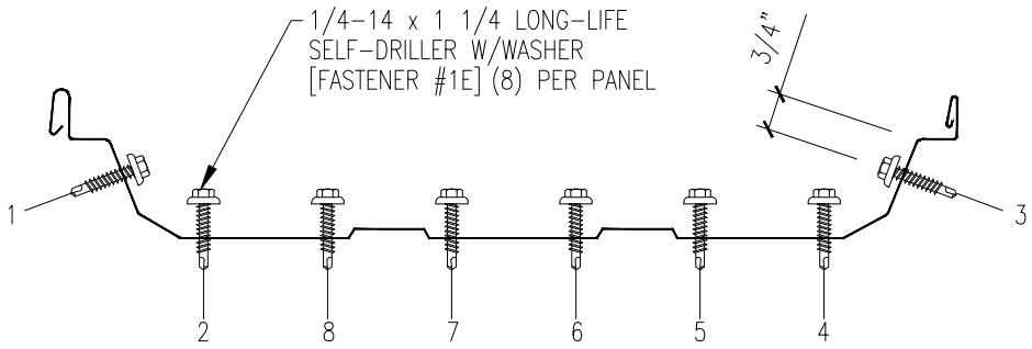
FASTENER SEQUENCE @ EAVE
