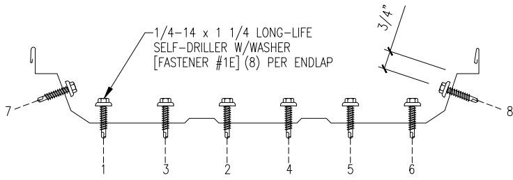
FASTENER SEQUENCE @ ENDLAP
