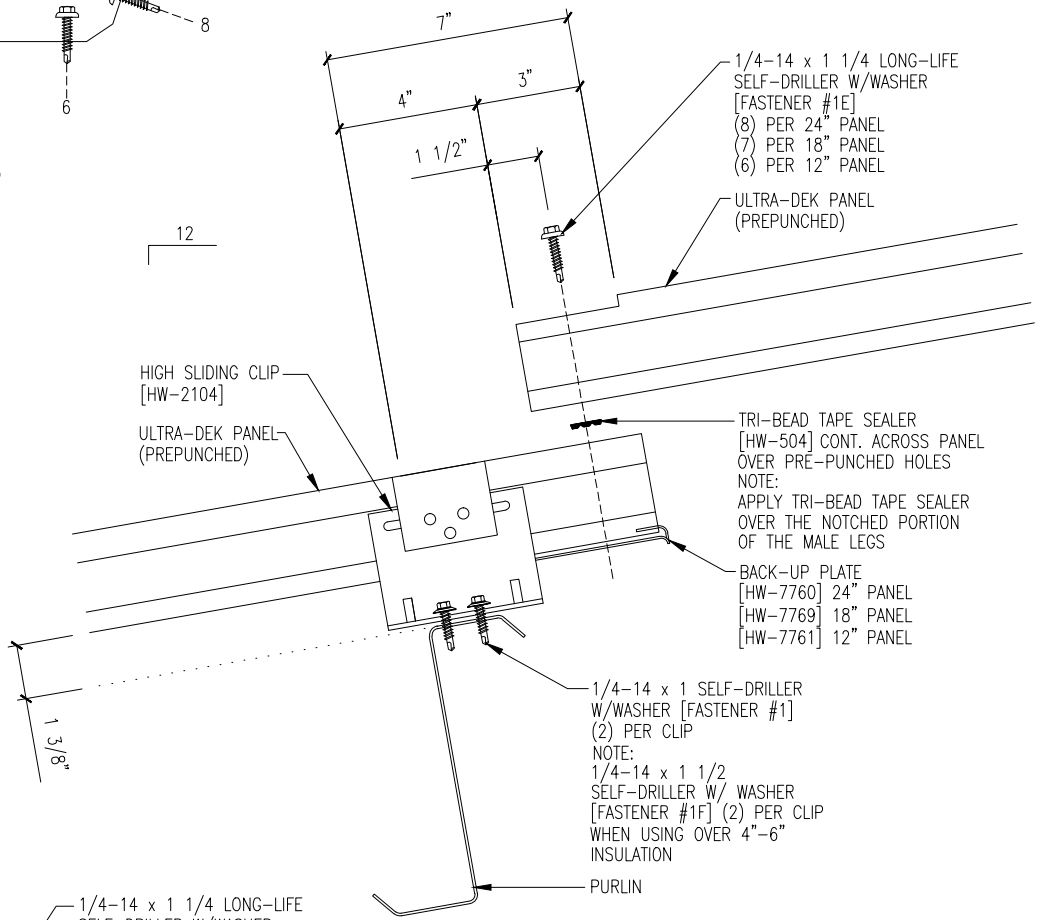
FASTENER SEQUENCE @ ENDLAP
