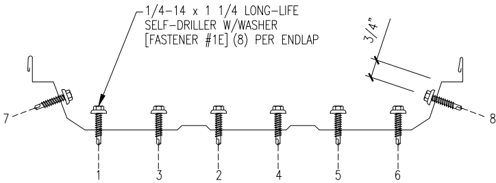
FASTENER SEQUENCE @ ENDLAP
