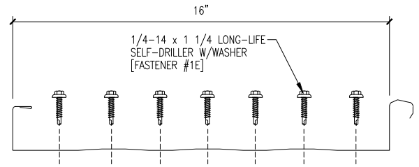
FASTENER LOCATIONS
