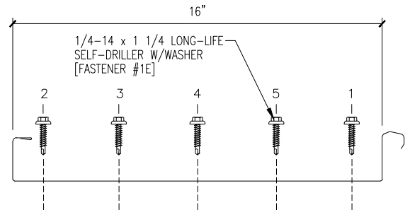
FASTENER INSTALLATION SEQUENCE
