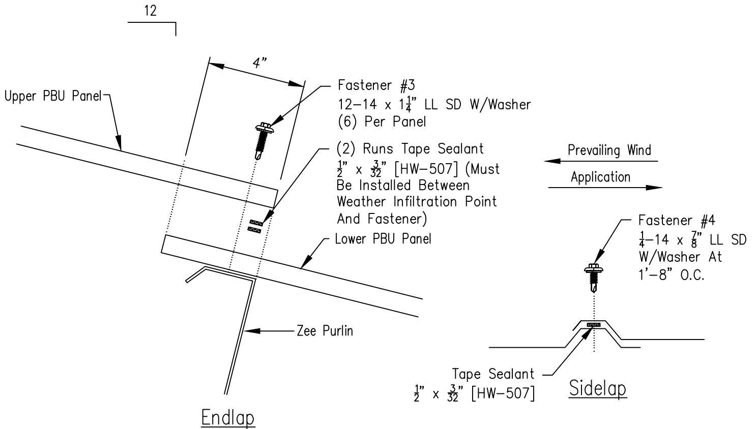
Endlap Sealant Detail
