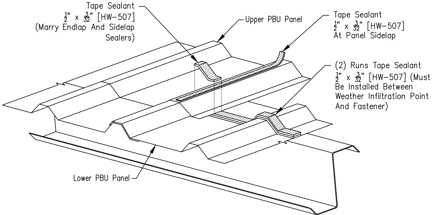
Endlap Sealant Detail
