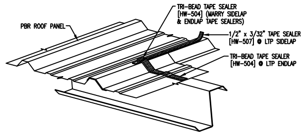
ENDLAP SEALANT DETAIL
