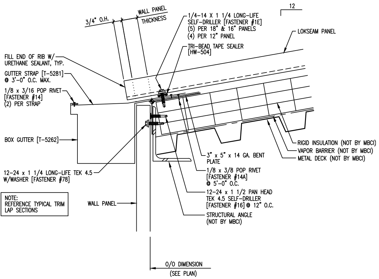
FASTENER SPACING @ EAVE
