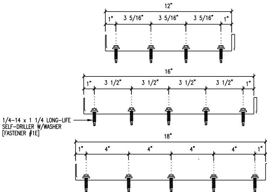
FASTENER SPACING @ EAVE
