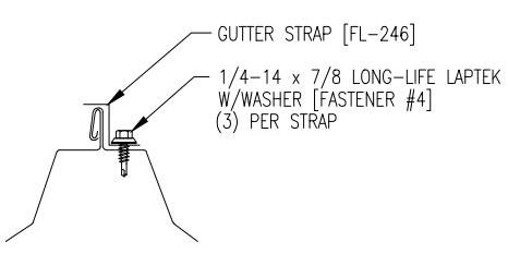
FASTENER SEQUENCE @ EAVE
