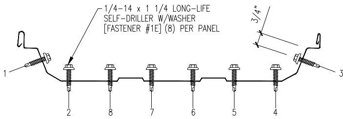
FASTENER SEQUENCE @ EAVE
