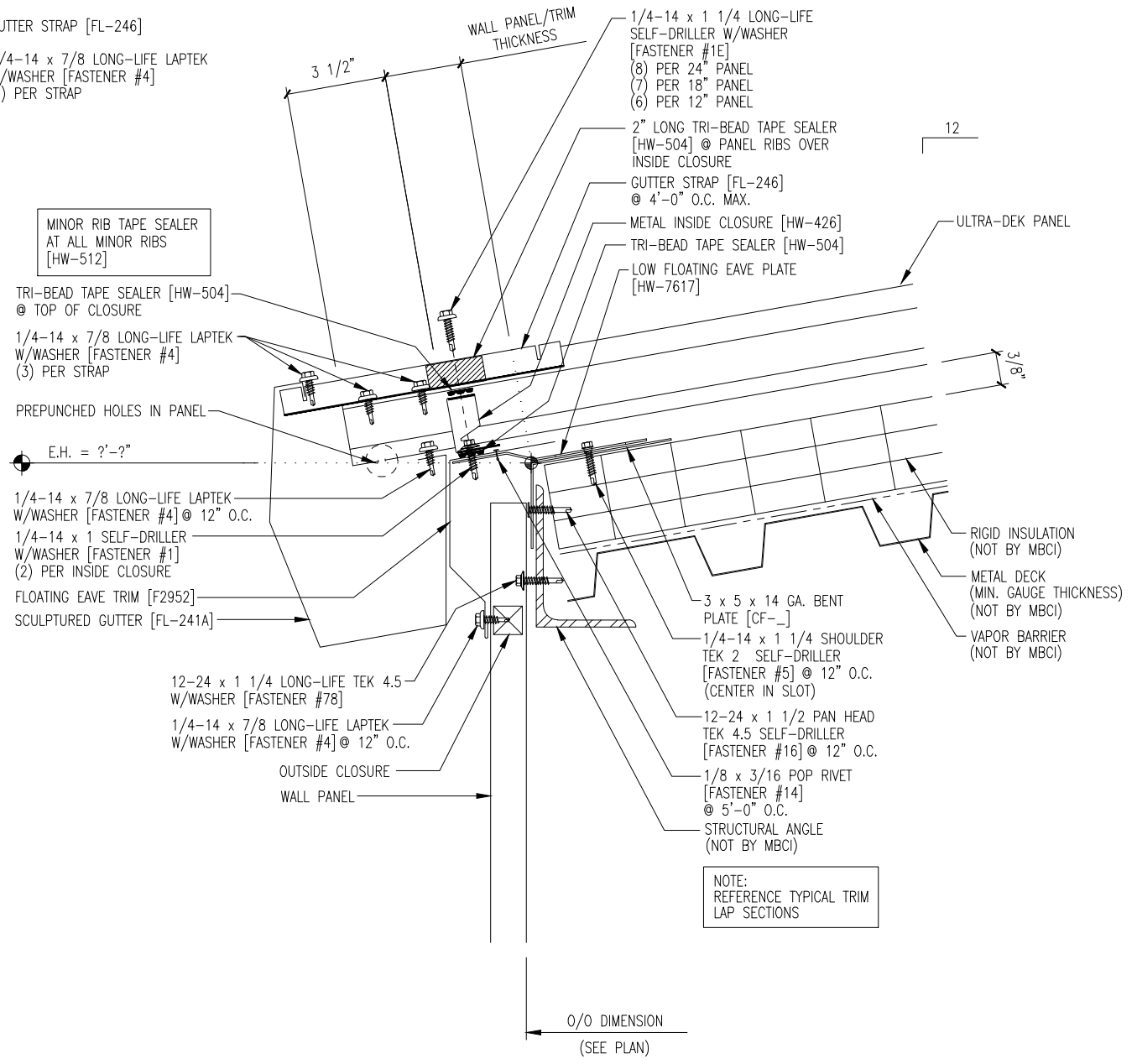
FASTENER SEQUENCE @ EAVE
