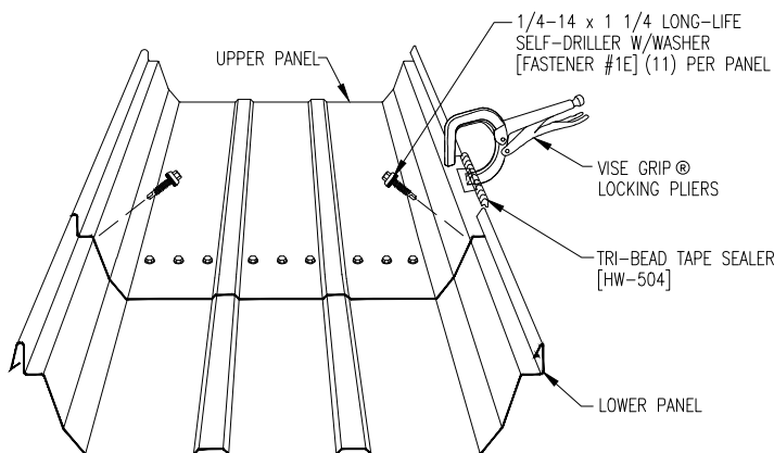
PANEL INSTALLATION SEQUENCE
