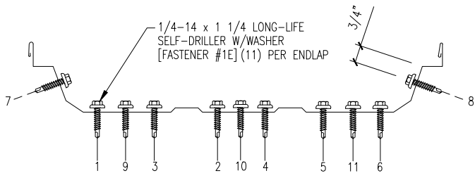
FASTENER SEQUENCE @ ENDLAP
