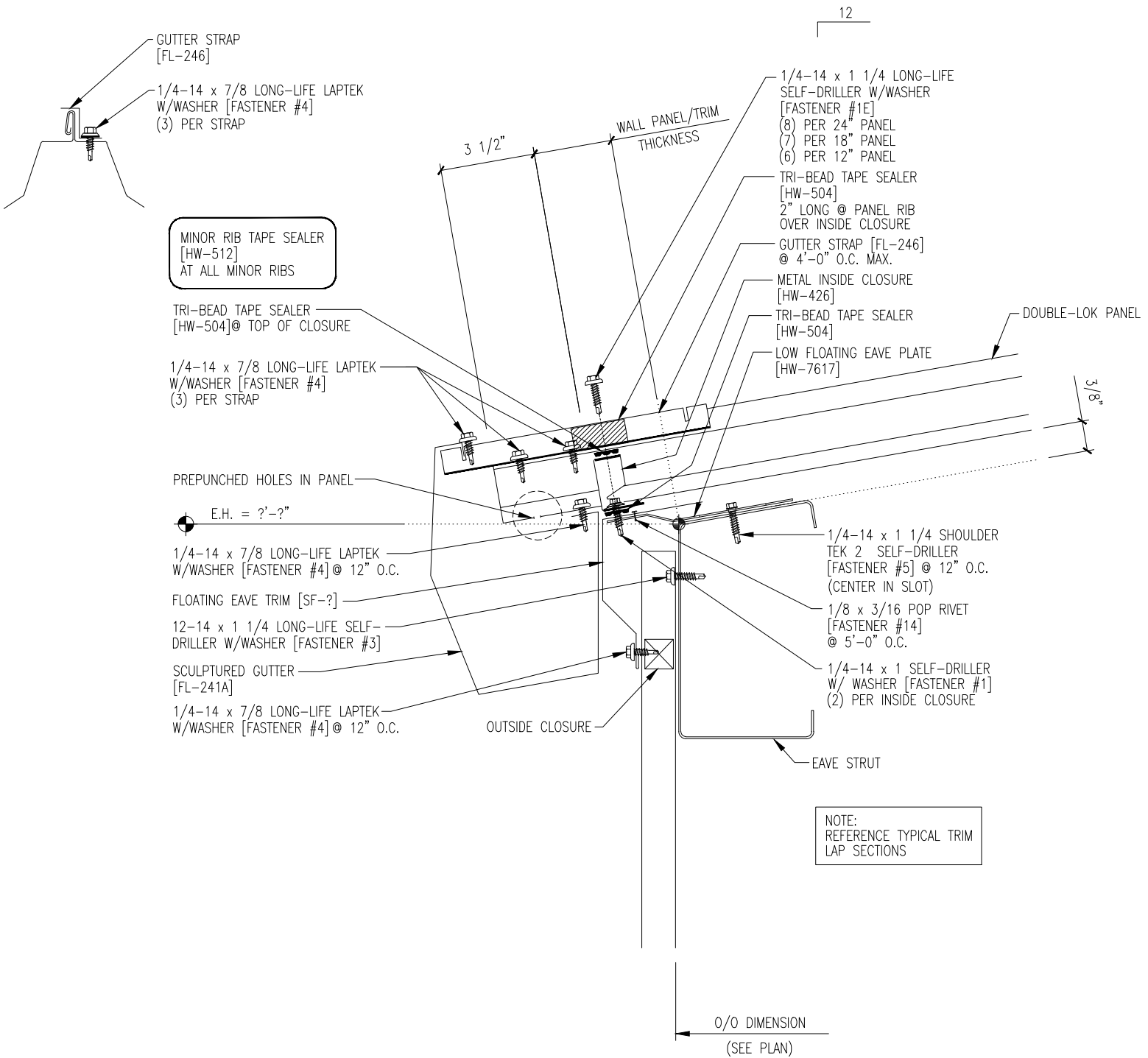
FASTENER SEQUENCE @ EAVE
