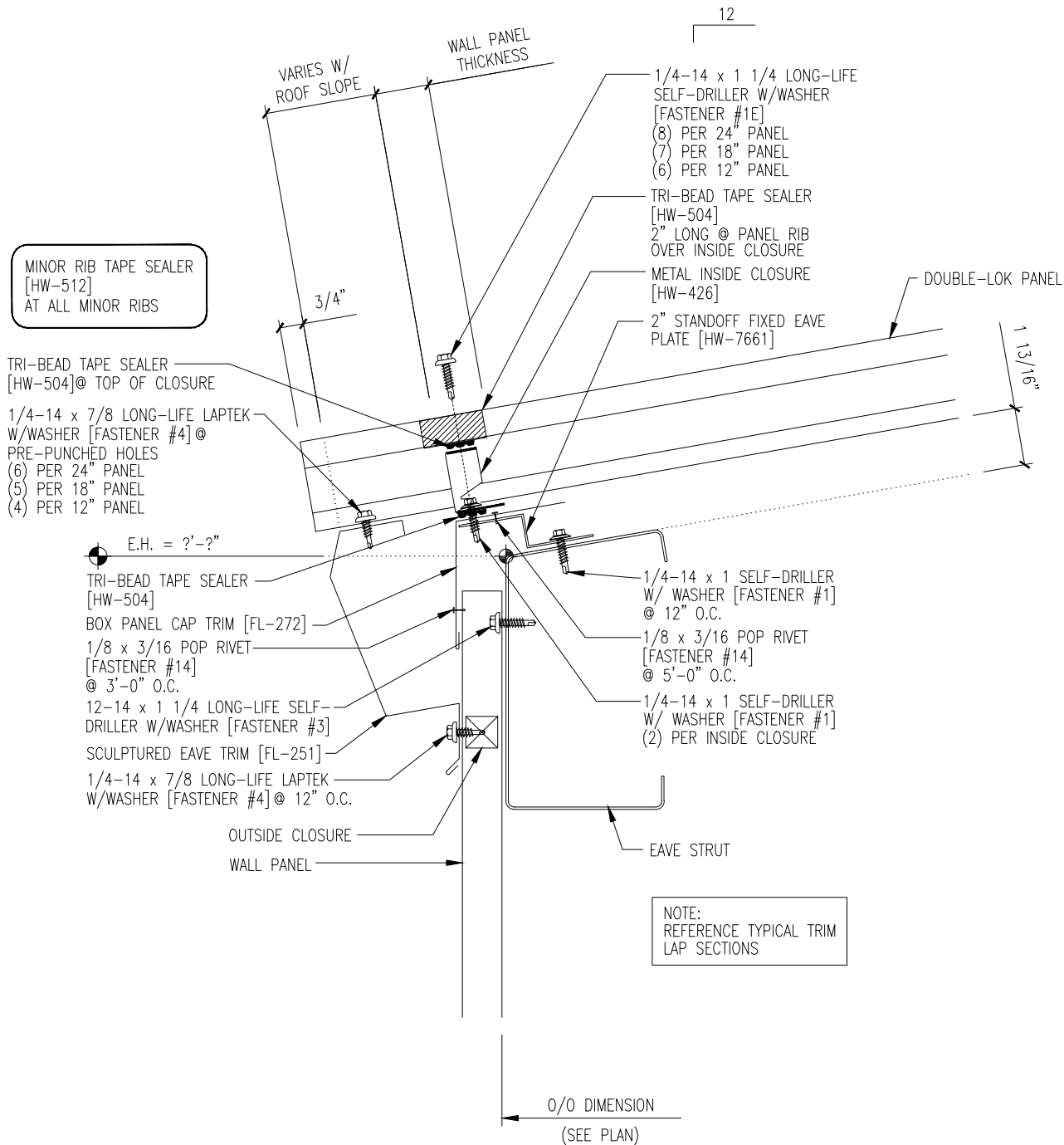
FASTENER SEQUENCE @ EAVE
