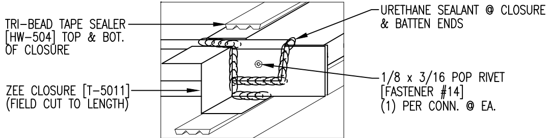
HIGH EAVE SEALANT DETAIL
