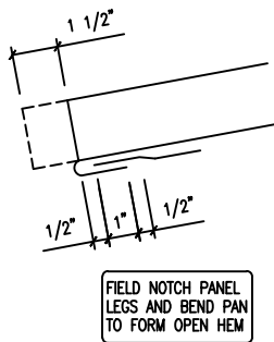
PANEL ENGAGEMENT DETAIL
