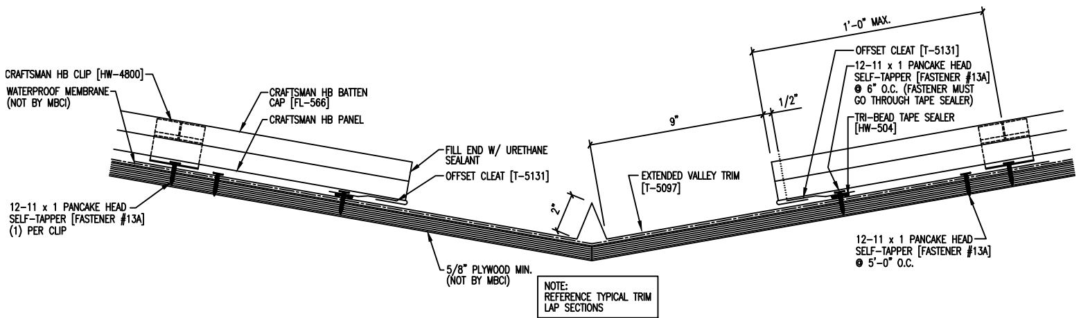
PANEL ENGAGEMENT DETAIL
