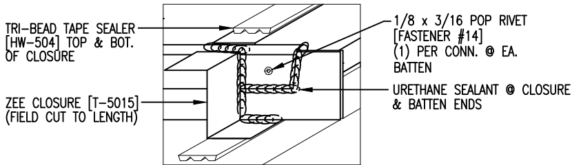
HIGH EAVE SEALANT DETAIL
